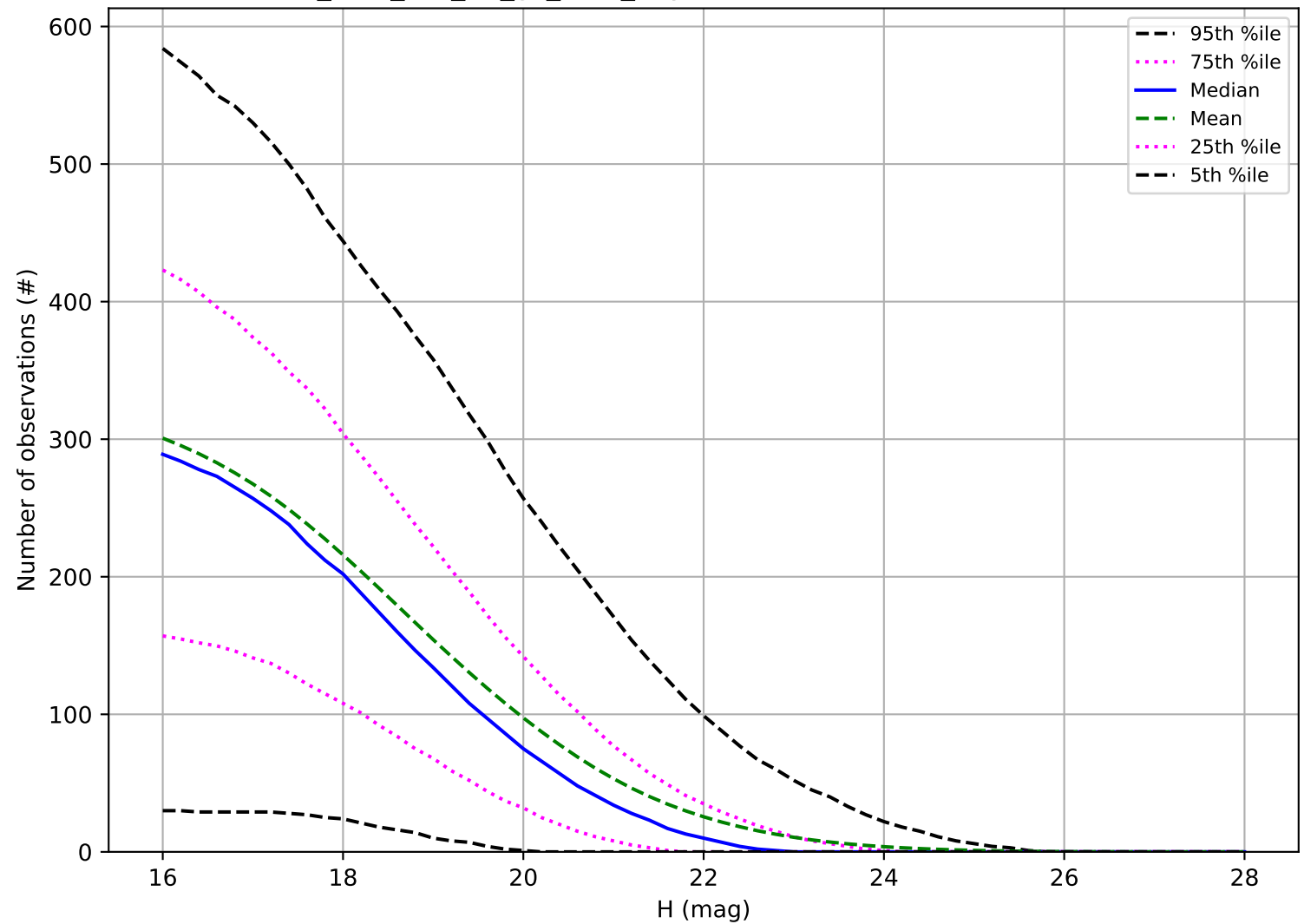
too_elab_r64_d2_gz_v3.4_10yrs: Number of observations NEO
