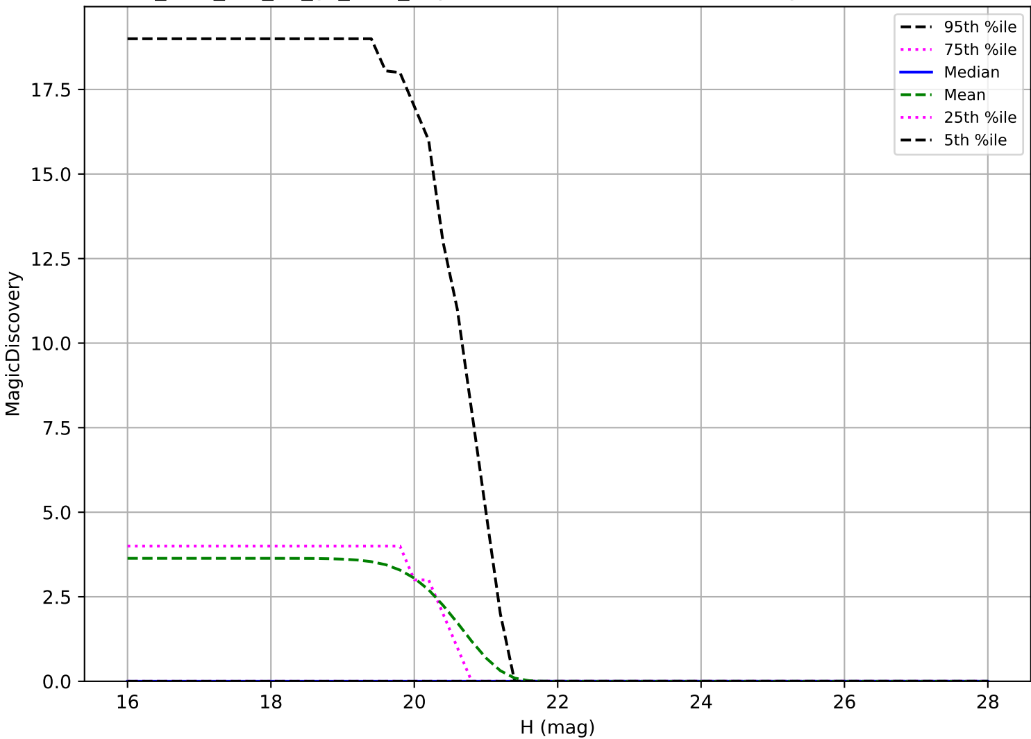
too_elab_r64_d2_gz_v3.4_10yrs: Vatira 6 detections in 60 nights detection loss
