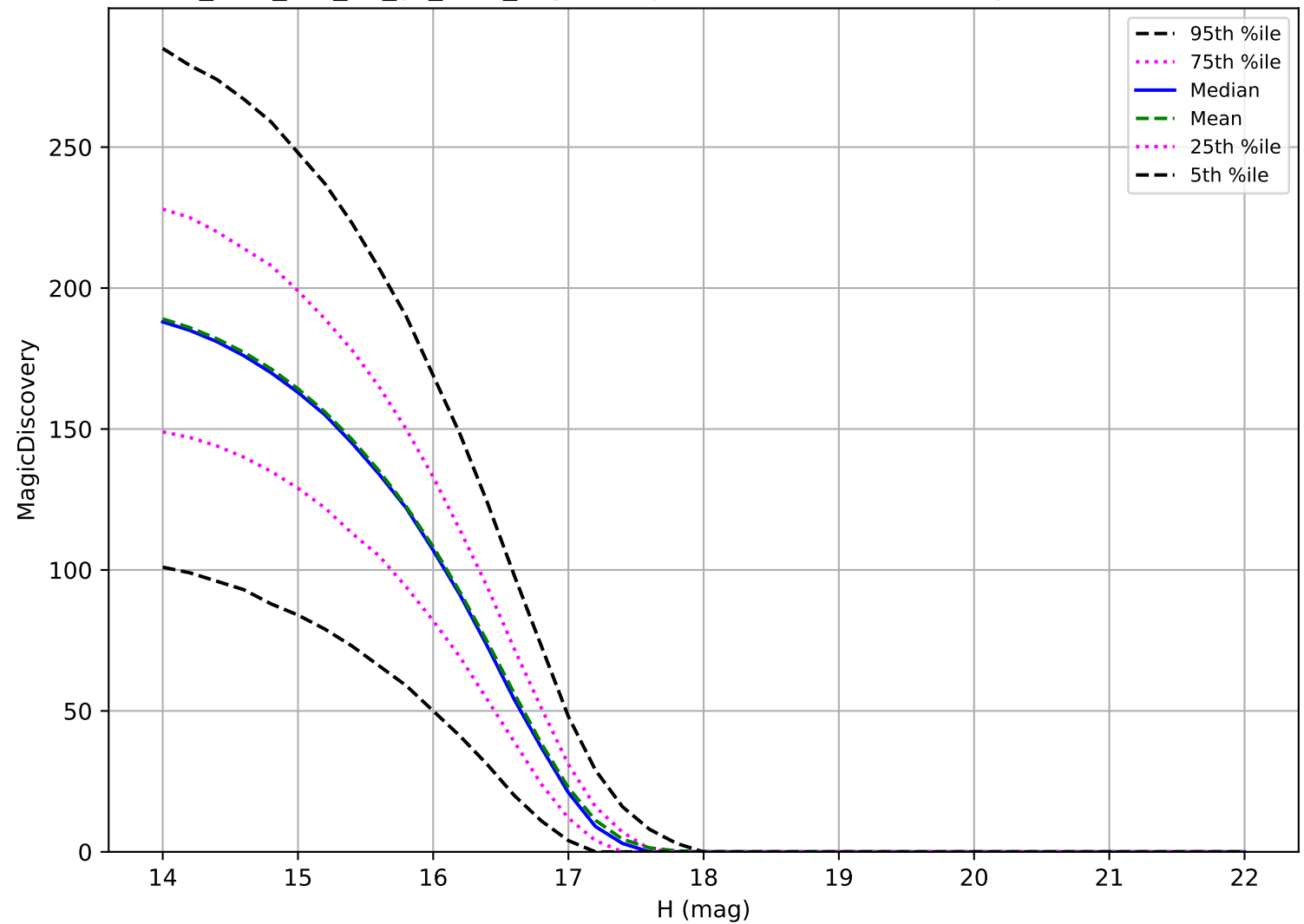
too_elab_r64_d2_gz_v3.4_10yrs: Trojan 6 detections in 60 nights detection loss
