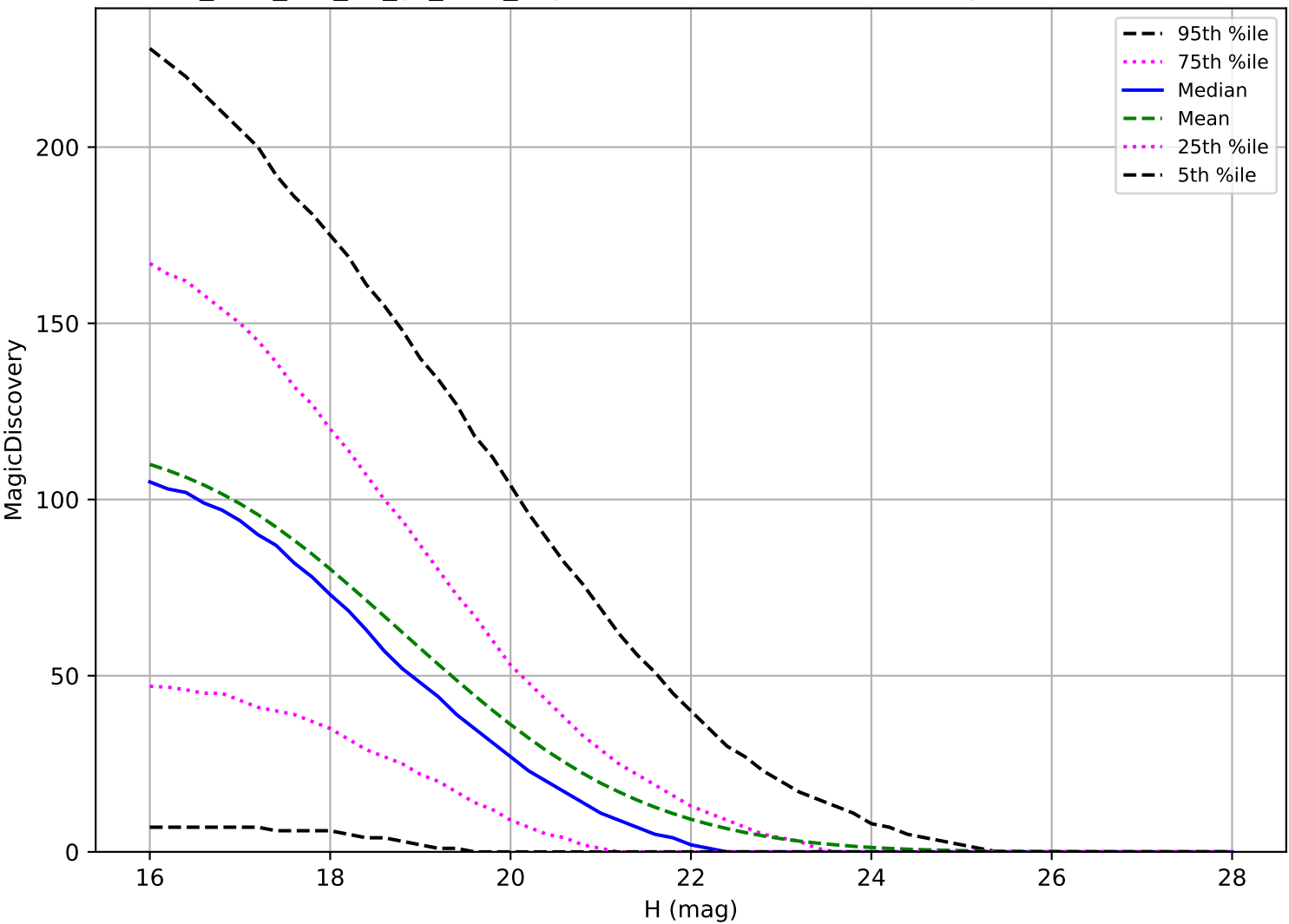
too_elab_r64_d2_gz_v3.4_10yrs: PHA 6 detections in 60 nights detection loss
