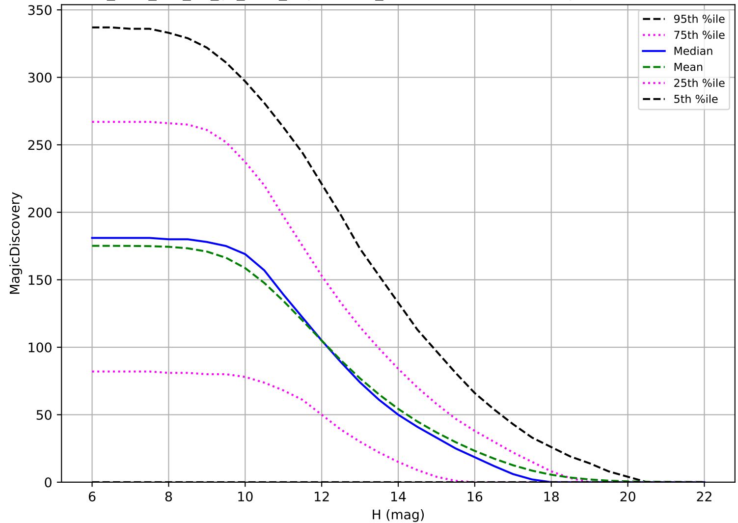
too_elab_r64_d2_gz_v3.4_10yrs: OCC_r5 6 detections in 60 nights detection loss
