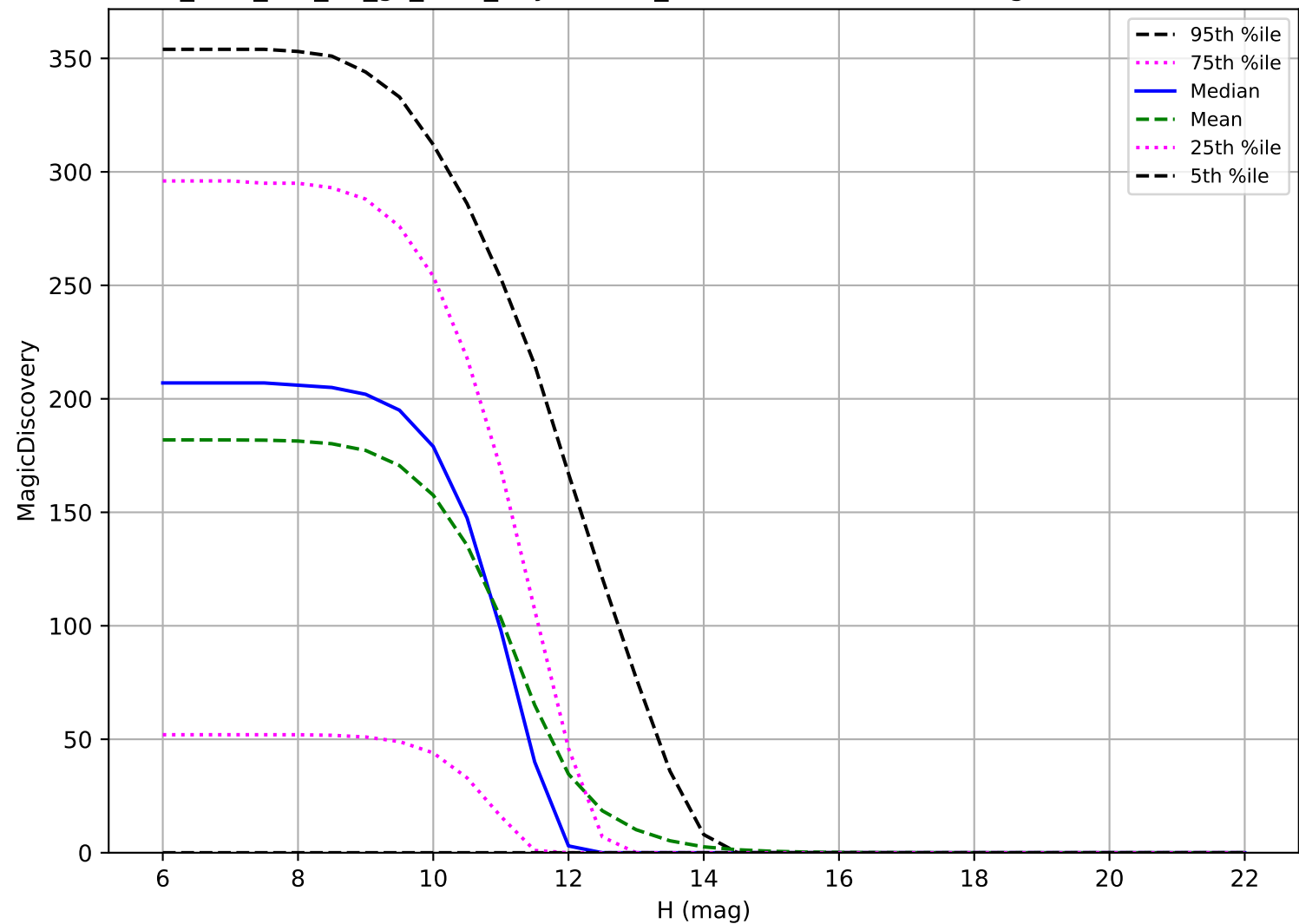
too_elab_r64_d2_gz_v3.4_10yrs: OCC_r20 6 detections in 60 nights detection loss
