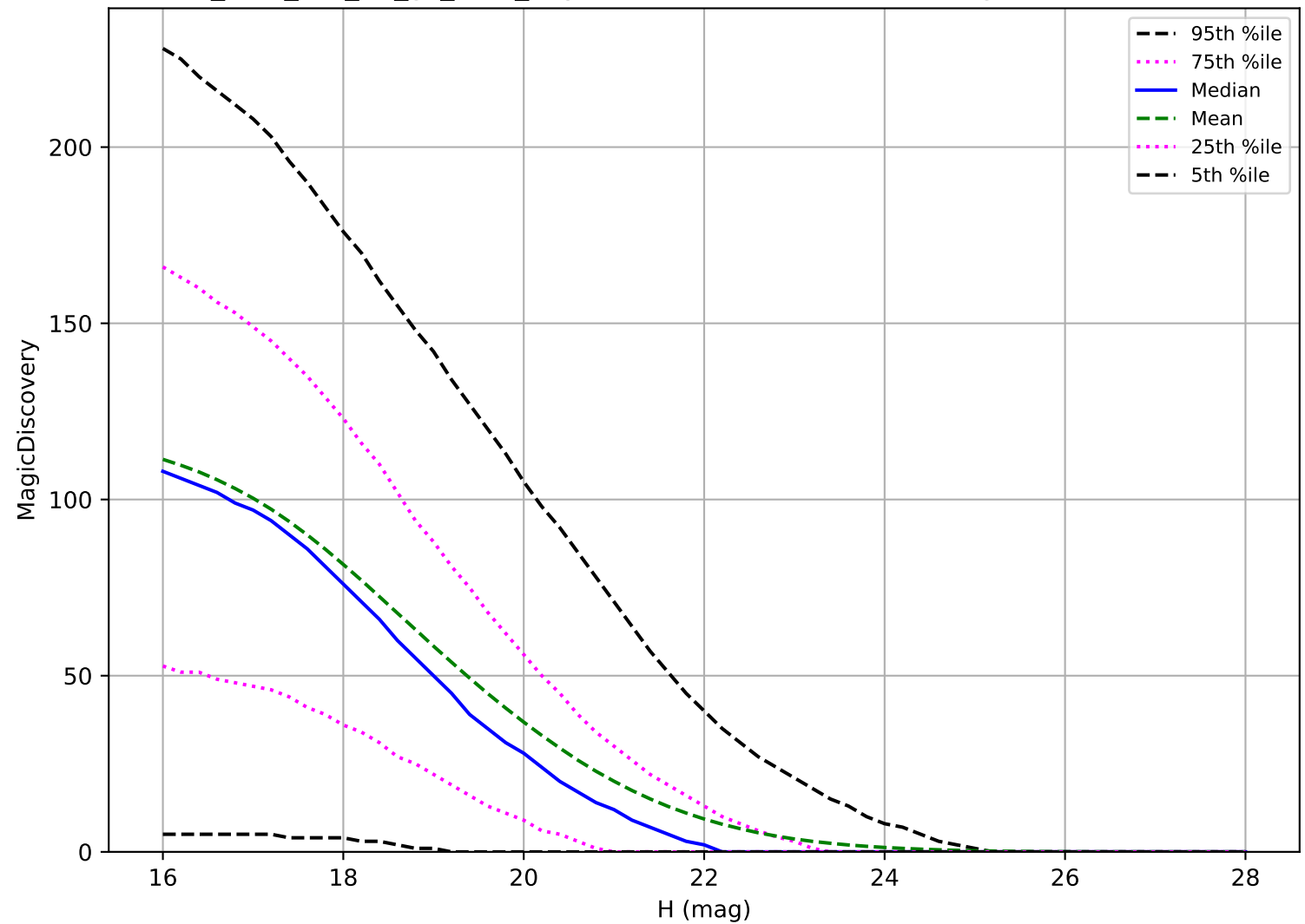
too_elab_r64_d2_gz_v3.4_10yrs: NEO 6 detections in 60 nights detection loss
