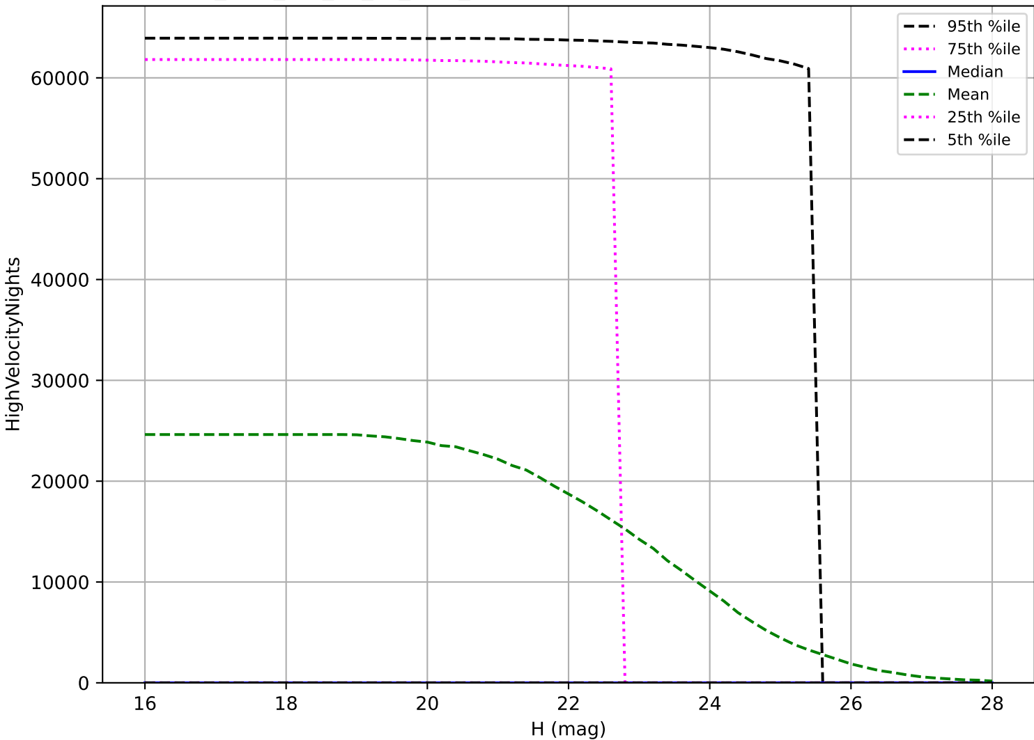
too_elab_r64_d2_gz_v3.4_10yrs: PHA High velocity pair detection loss
