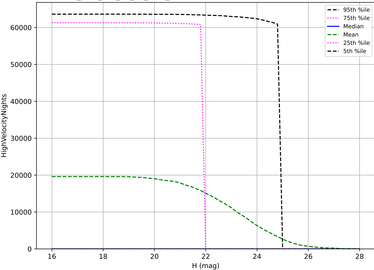
too_elab_r64_d2_gz_v3.4_10yrs: NEO High velocity pair detection loss
