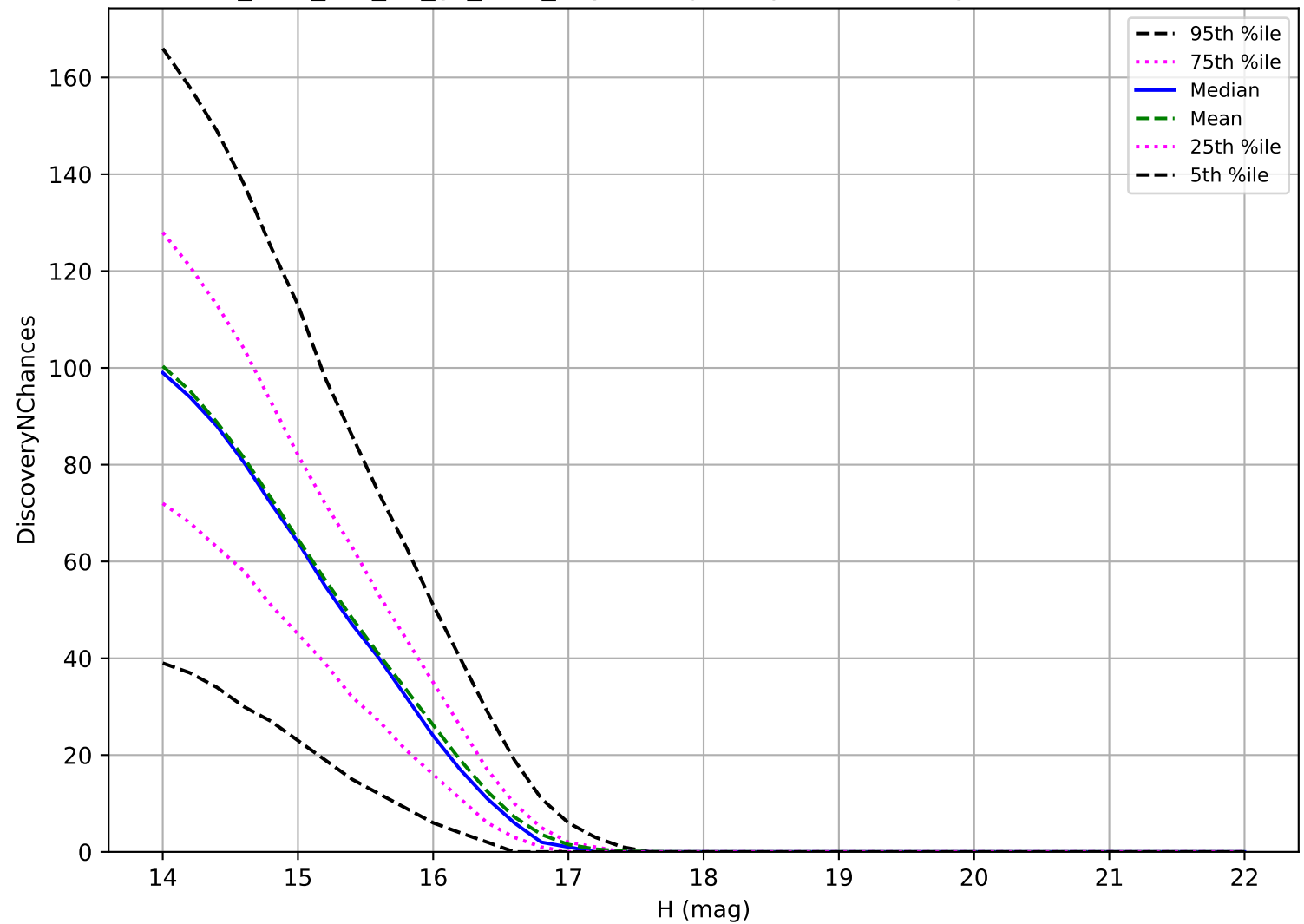
too_elab_r64_d2_gz_v3.4_10yrs: Trojan 3 pairs in 15 nights detection loss
