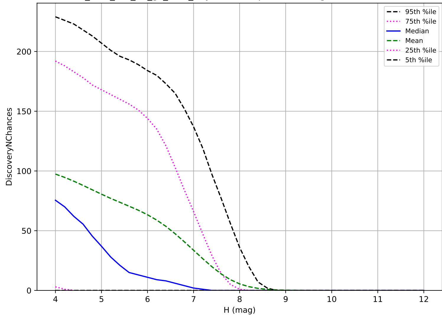
too_elab_r64_d2_gz_v3.4_10yrs: TNO 3 pairs in 15 nights detection loss
