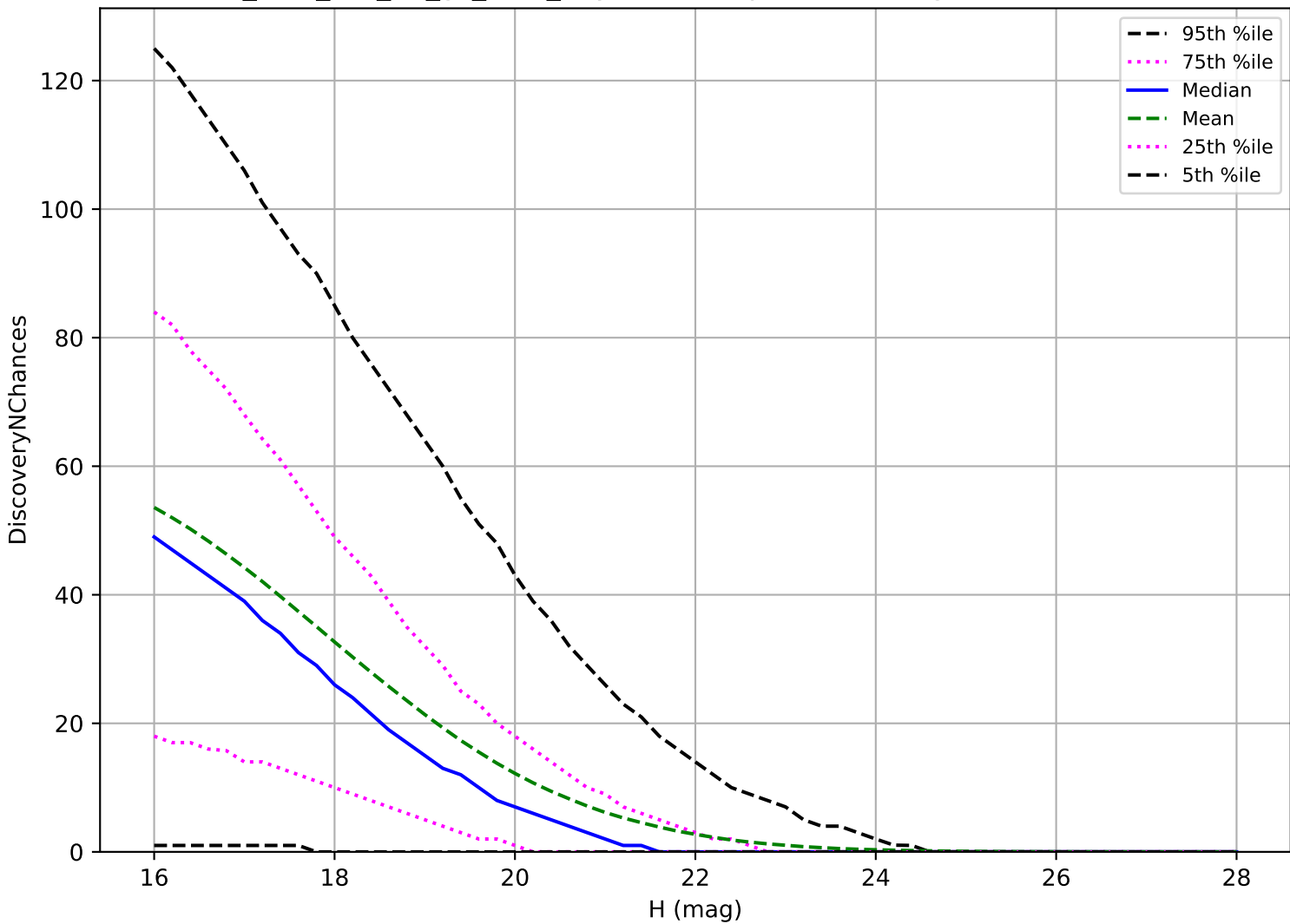
too_elab_r64_d2_gz_v3.4_10yrs: PHA 3 pairs in 15 nights detection loss
