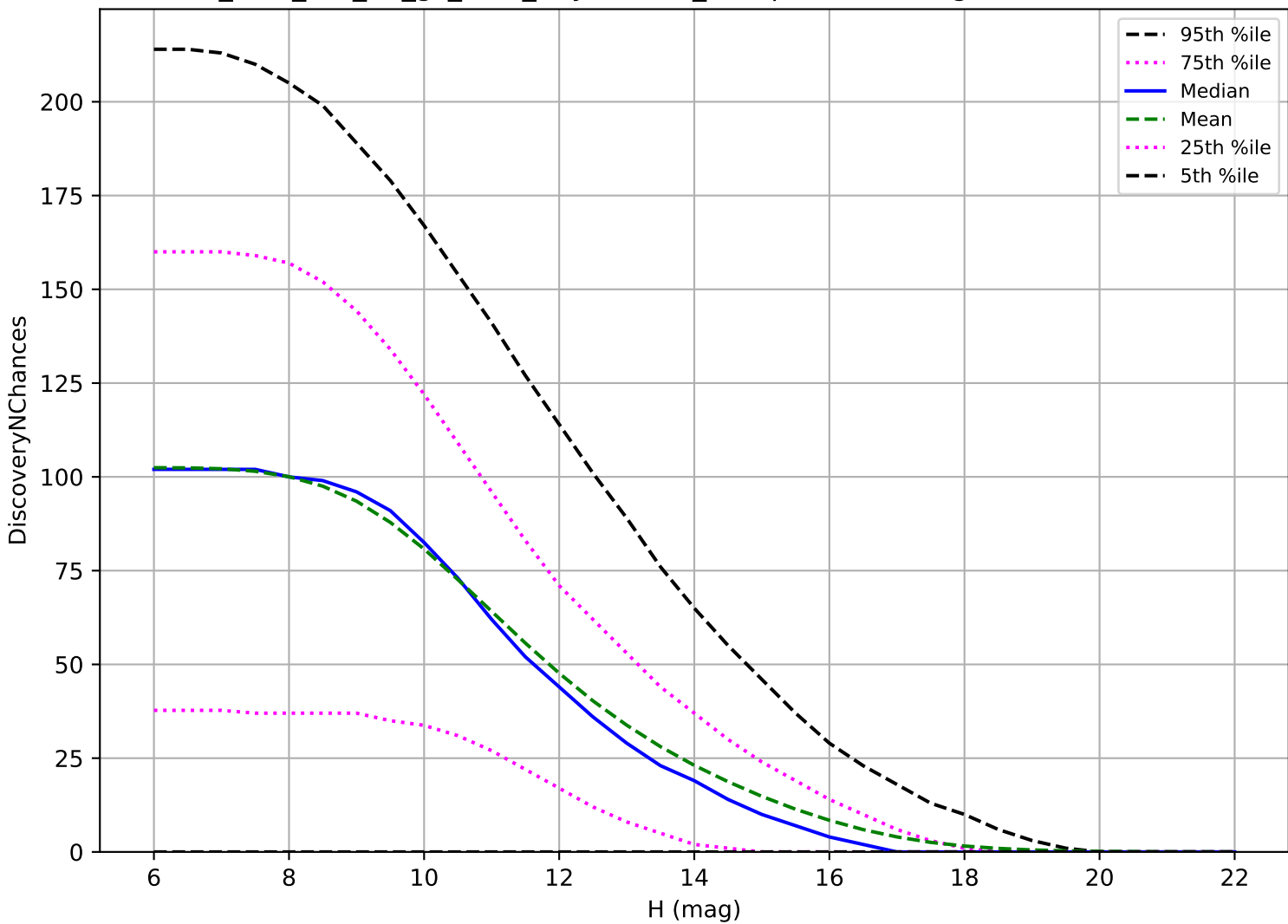
too_elab_r64_d2_gz_v3.4_10yrs: OCC_r5 3 pairs in 15 nights detection loss
