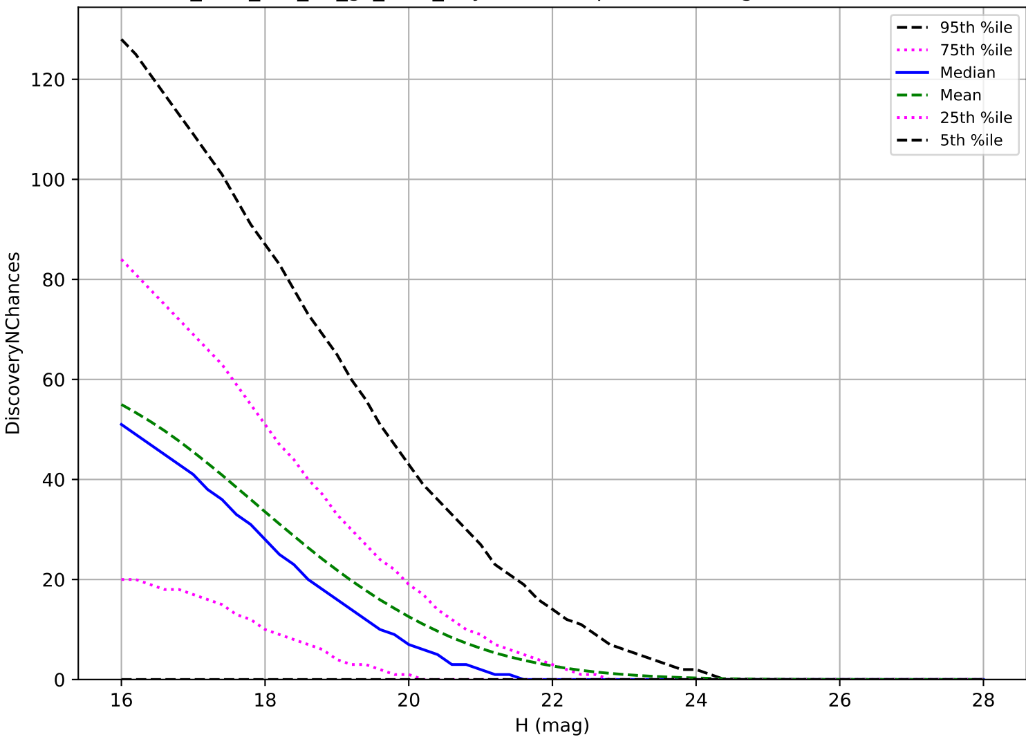
too_elab_r64_d2_gz_v3.4_10yrs: NEO 3 pairs in 15 nights detection loss
