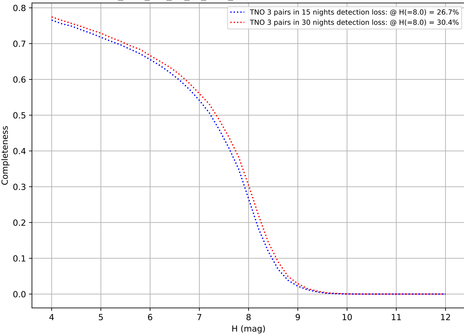
too_elab_r64_d2_gz_v3.4_10yrs: DifferentialCompleteness
