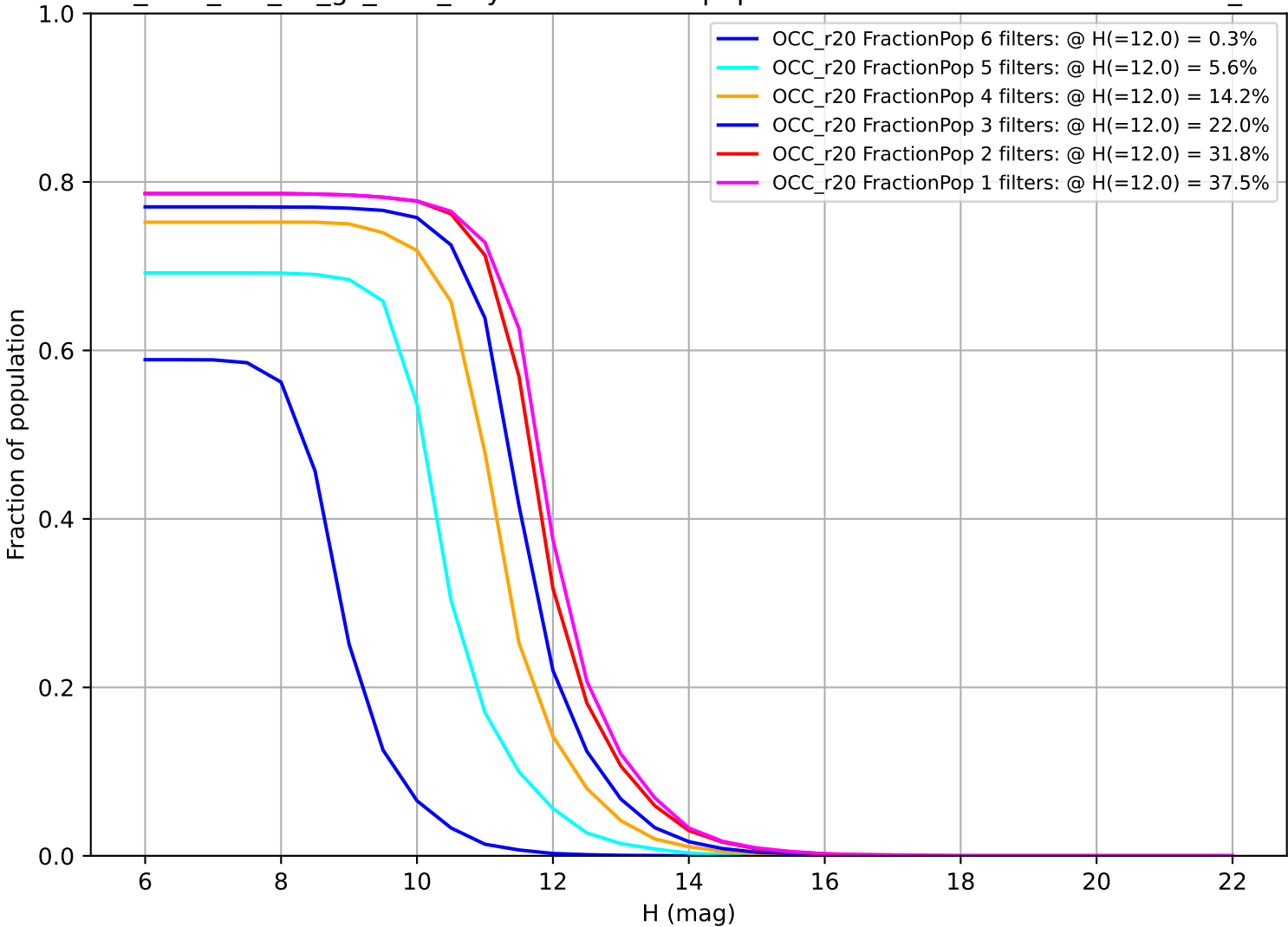
too_elab_r64_d2_gz_v3.4_10yrs: Fraction of population with colors in X filters OCC_r20
