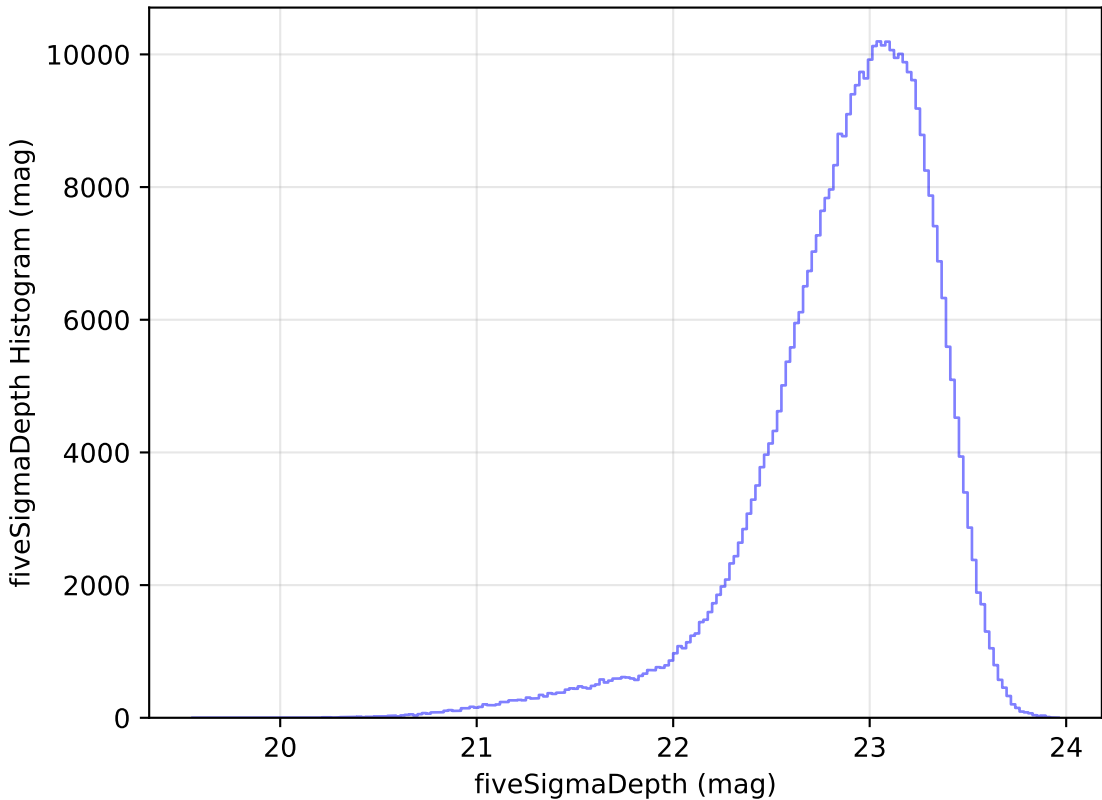
too_elab_r64_d2_gz_v3.4_10yrs z: fiveSigmaDepth Histogram
