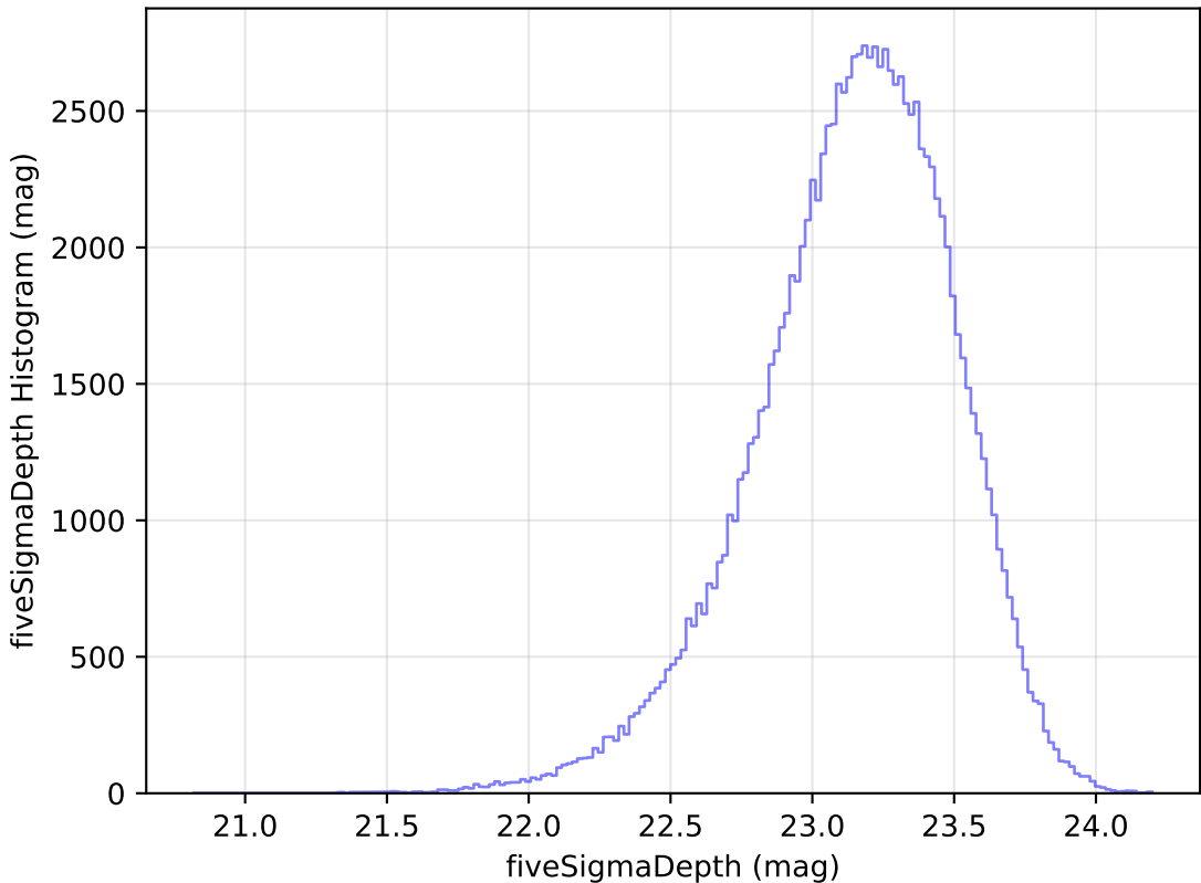
too_elab_r64_d2_gz_v3.4_10yrs u: fiveSigmaDepth Histogram
