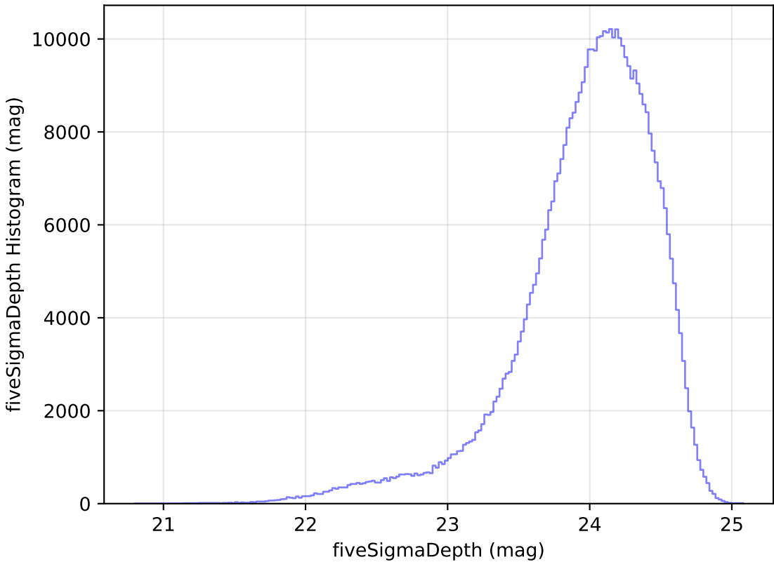
too_elab_r64_d2_gz_v3.4_10yrs r: fiveSigmaDepth Histogram
