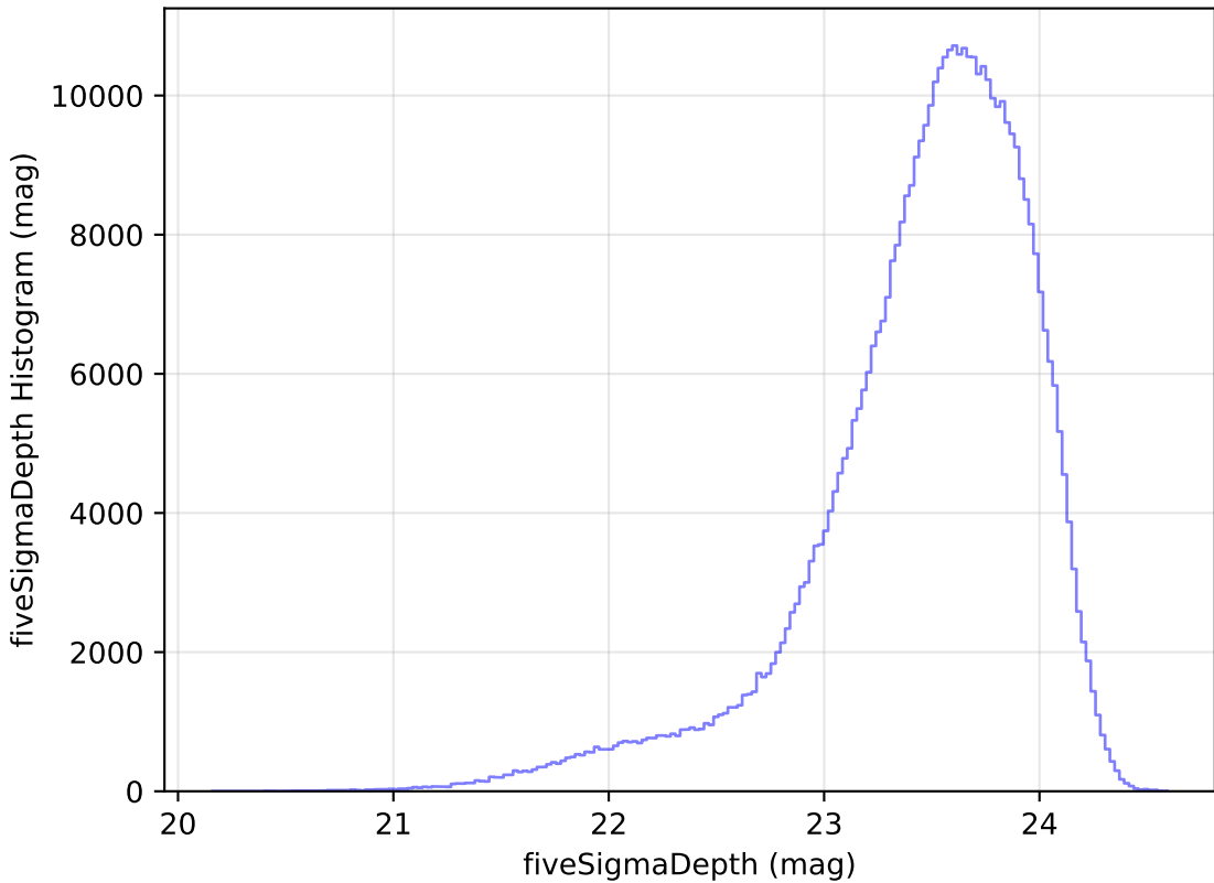
too_elab_r64_d2_gz_v3.4_10yrs i: fiveSigmaDepth Histogram
