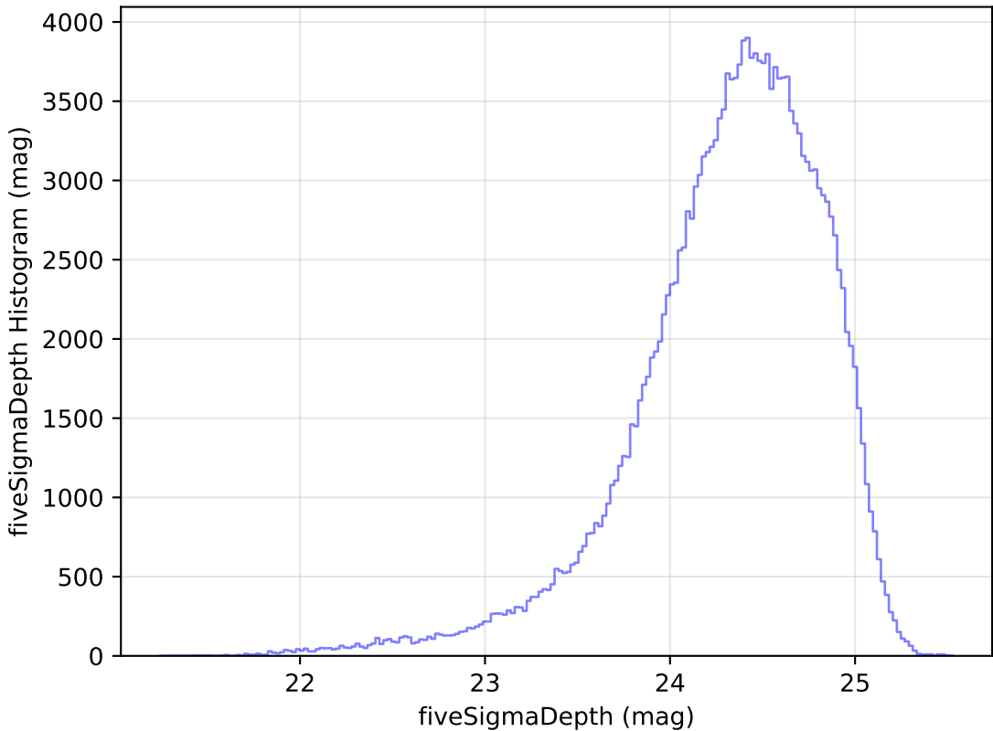
too_elab_r64_d2_gz_v3.4_10yrs g: fiveSigmaDepth Histogram
