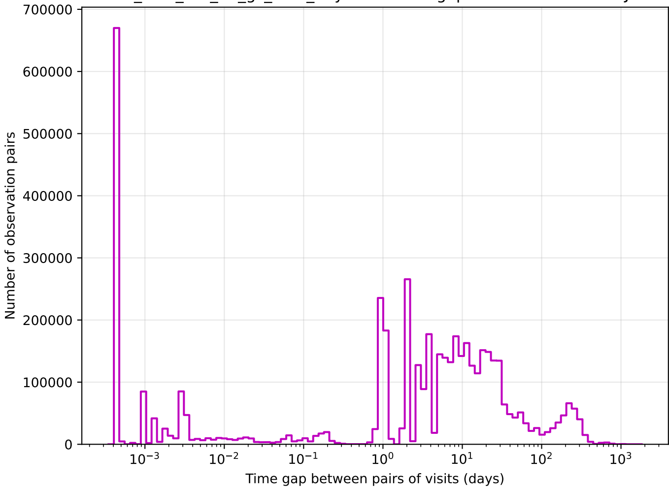
too_elab_r64_d2_gz_v3.4_10yrs z band: Tgaps observationStartMJD
