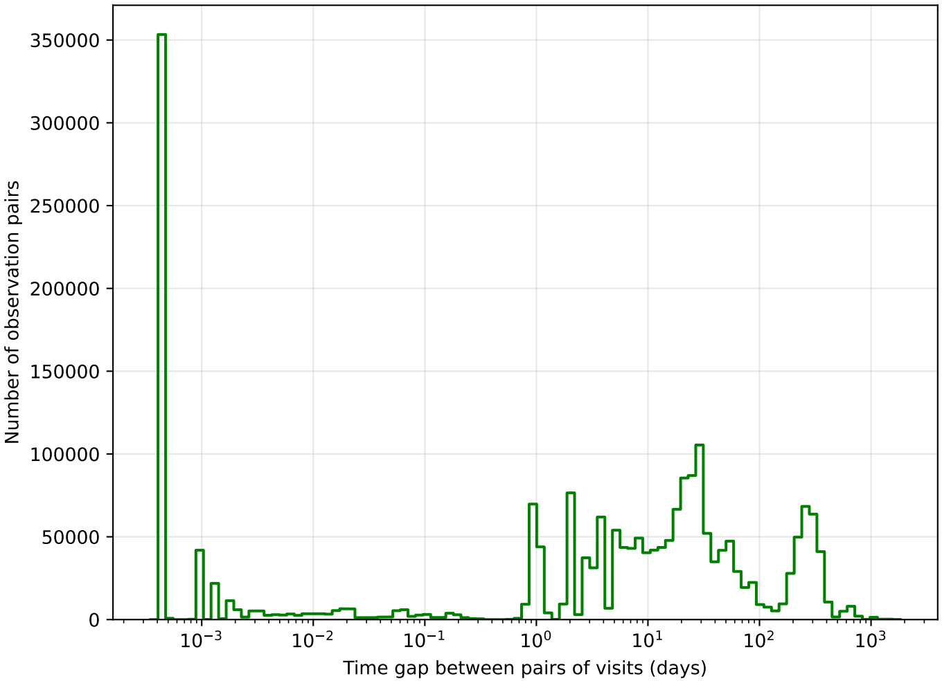
too_elab_r64_d2_gz_v3.4_10yrs g band: Tgaps observationStartMJD
