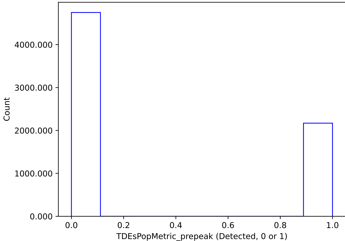
too_elab_r64_d2_gz_v3.4_10yrs : TDEsPopMetric_prepeak
