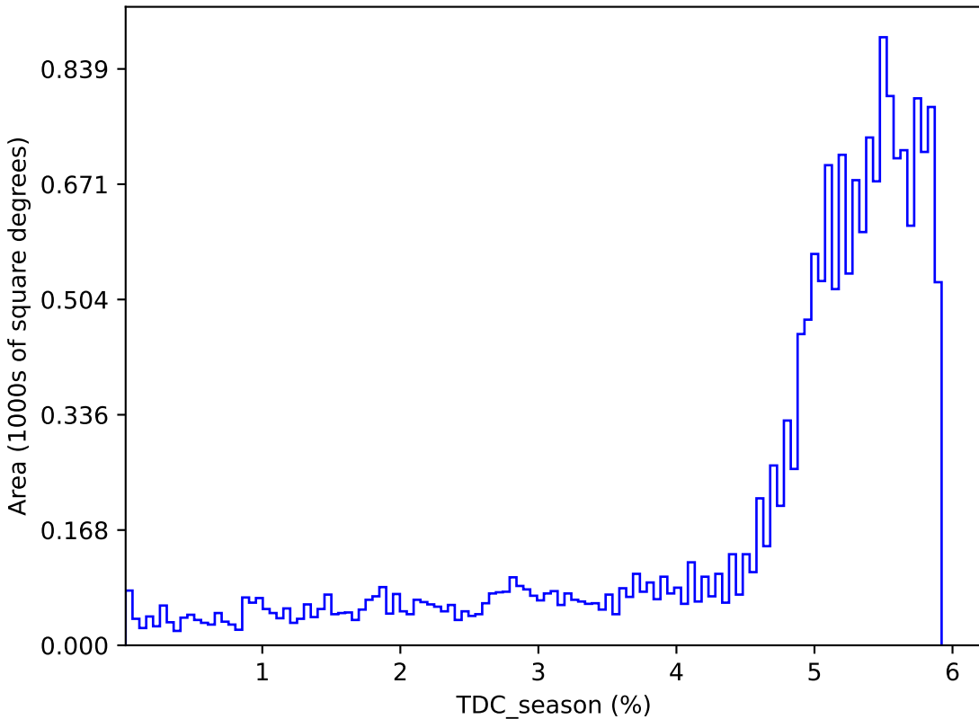
too_elab_r64_d2_gz_v3.4_10yrs : TDC_season
