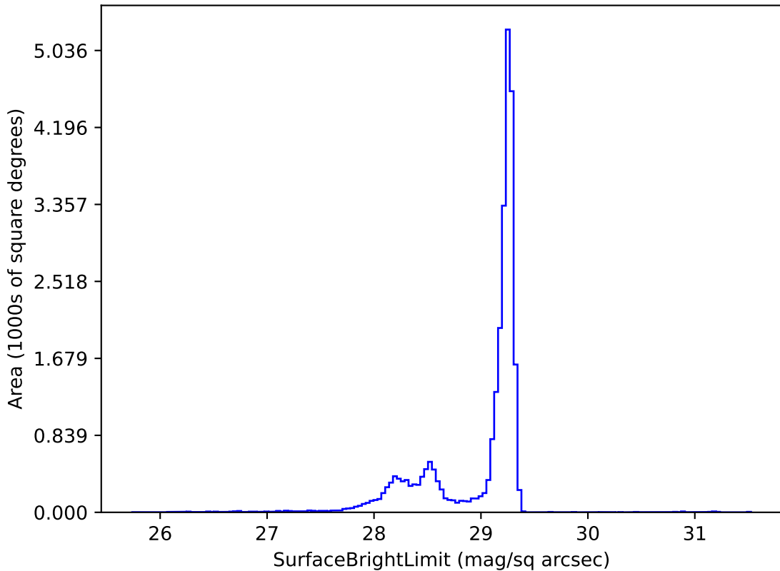
too_elab_r64_d2_gz_v3.4_10yrs z: SurfaceBrightLimit
