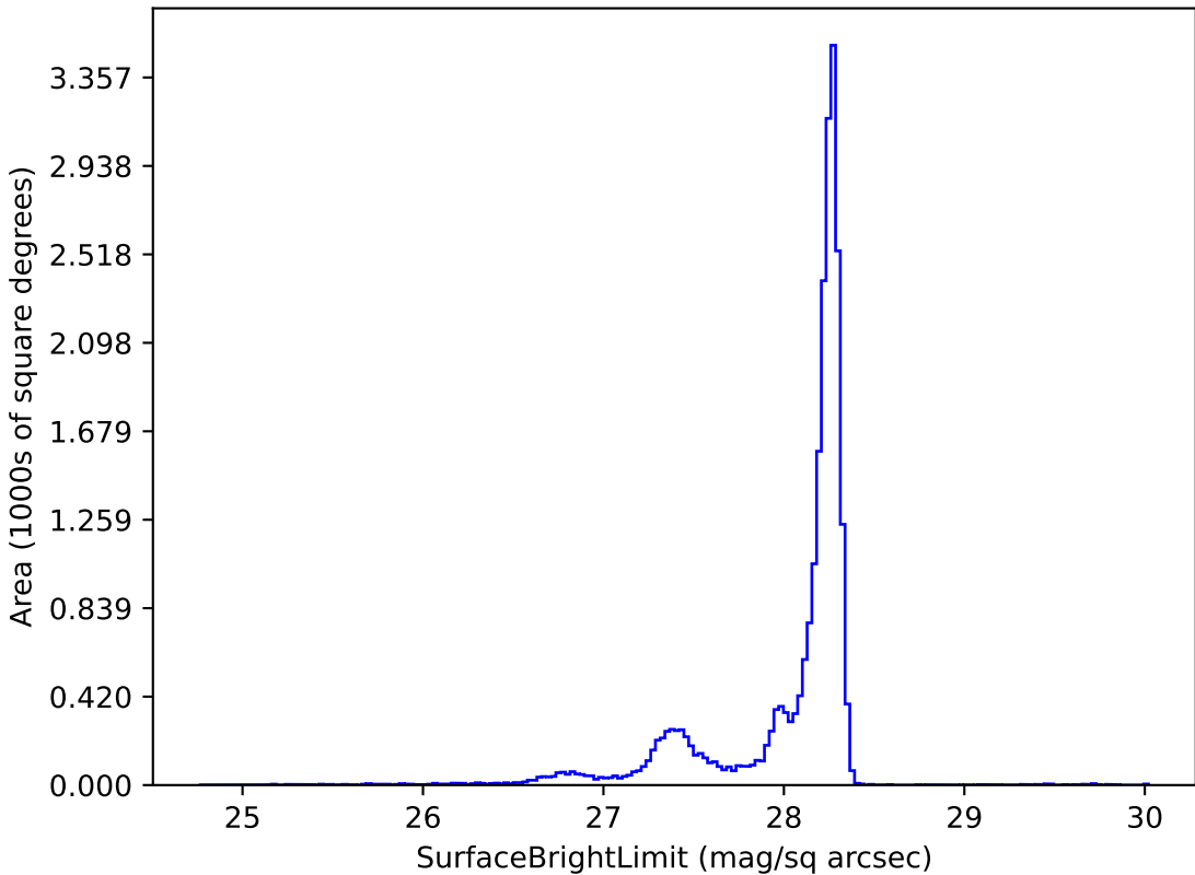
too_elab_r64_d2_gz_v3.4_10yrs y: SurfaceBrightLimit
