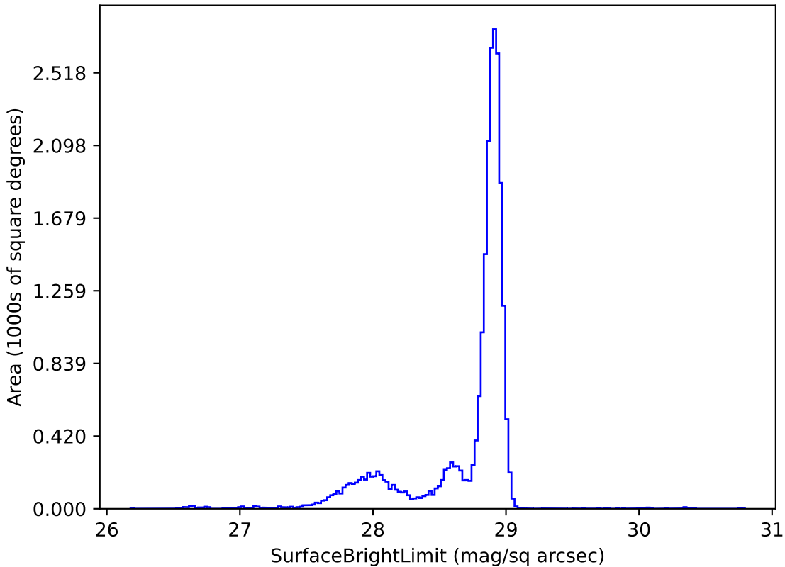
too_elab_r64_d2_gz_v3.4_10yrs u: SurfaceBrightLimit
