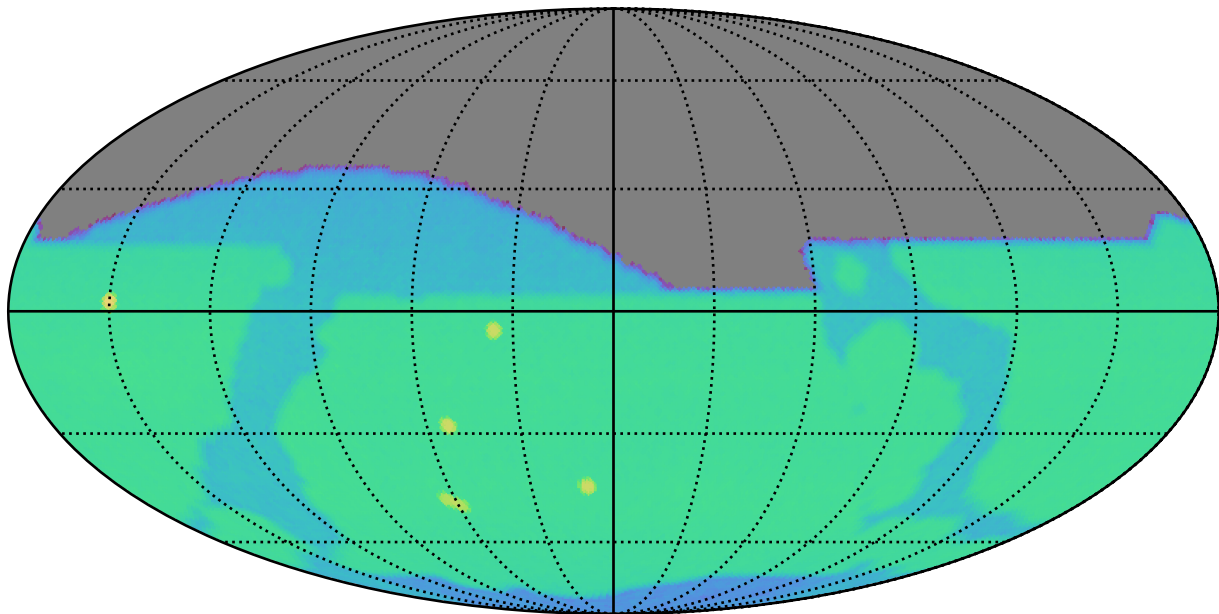
too_elab_r64_d2_gz_v3.4_10yrs i: SurfaceBrightLimit
