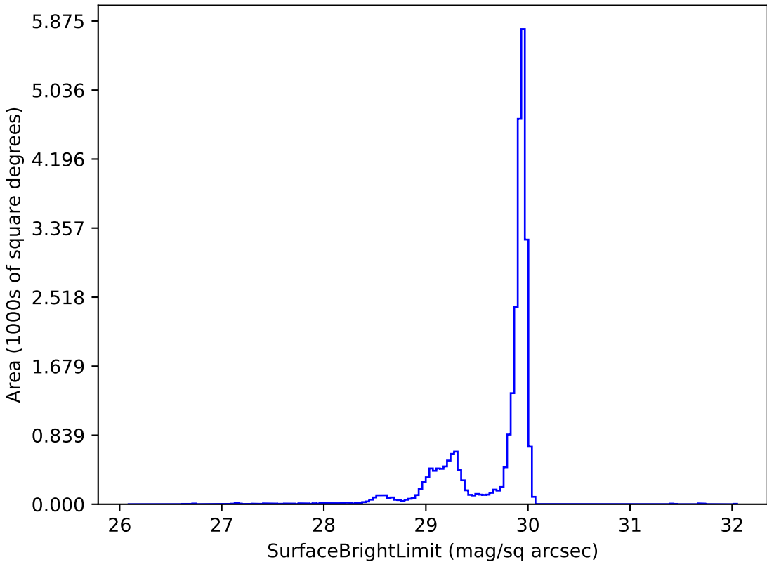
too_elab_r64_d2_gz_v3.4_10yrs i: SurfaceBrightLimit
