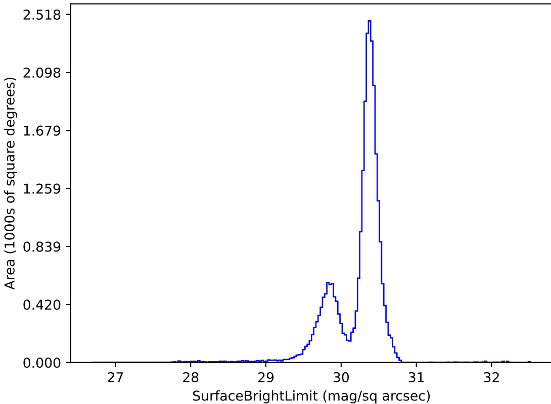
too_elab_r64_d2_gz_v3.4_10yrs g: SurfaceBrightLimit
