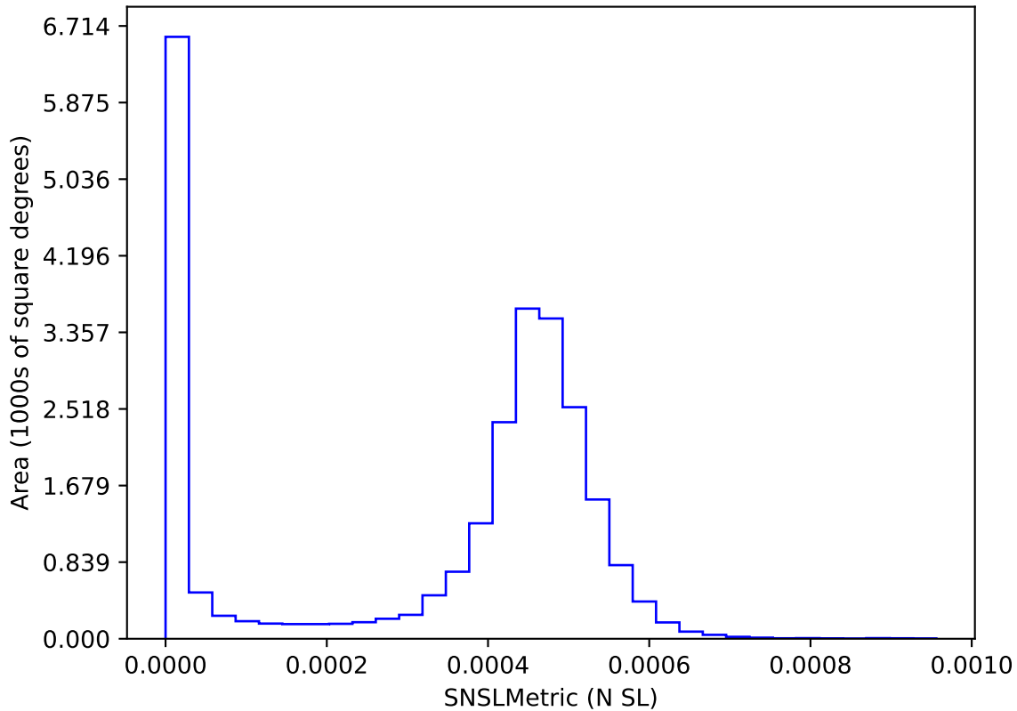
too_elab_r64_d2_gz_v3.4_10yrs : SNSLMetric
