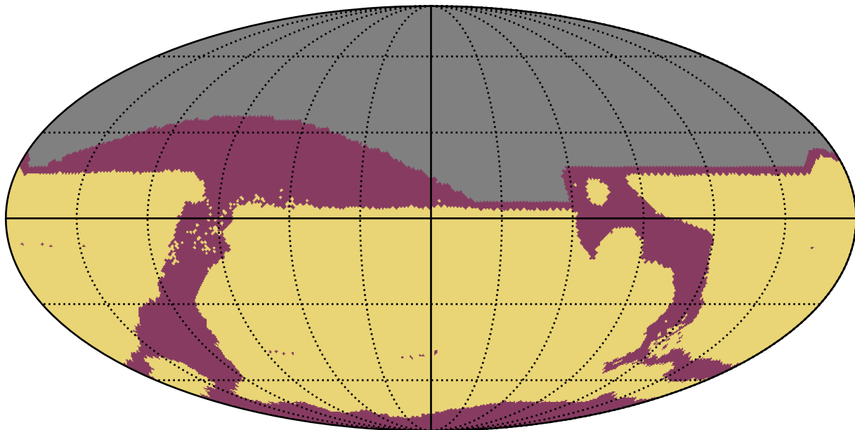
too_elab_r64_d2_gz_v3.4_10yrs : RapidRevisits
