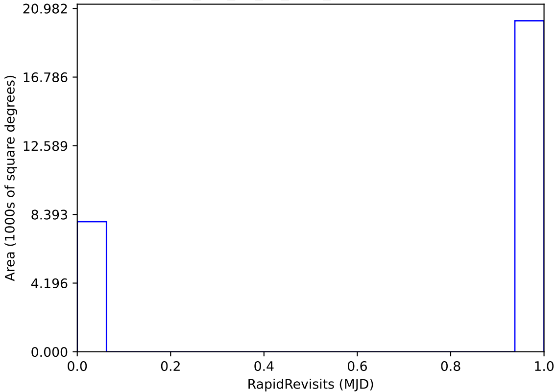
too_elab_r64_d2_gz_v3.4_10yrs : RapidRevisits
