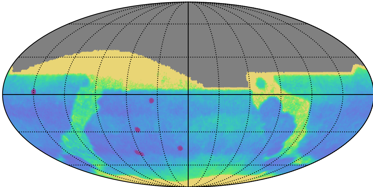
too_elab_r64_d2_gz_v3.4_10yrs : Proper Motion Uncert @ 24.0
