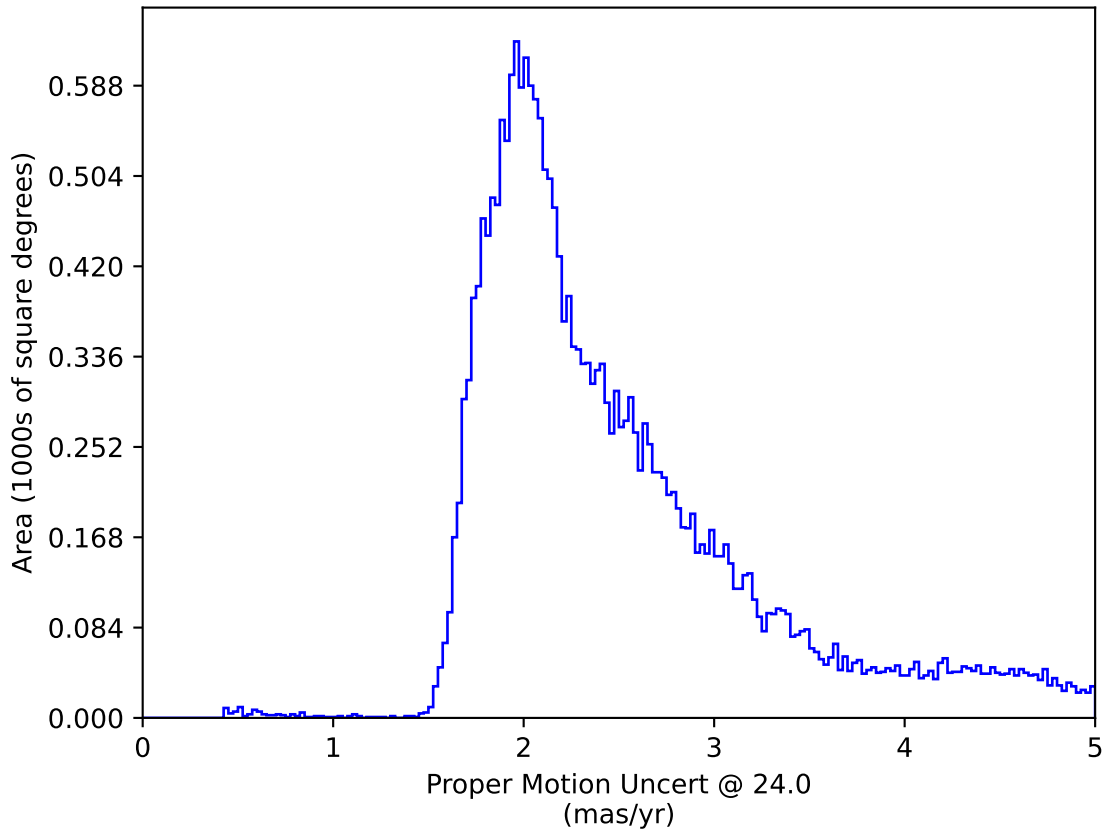
too_elab_r64_d2_gz_v3.4_10yrs : Proper Motion Uncert @ 24.0
