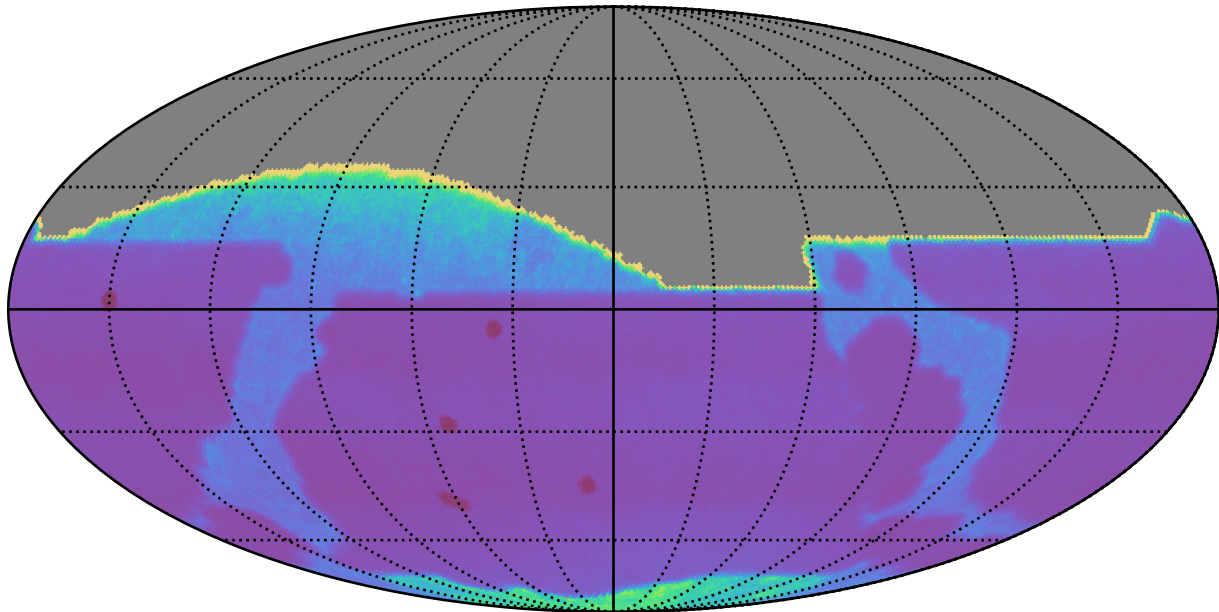
too_elab_r64_d2_gz_v3.4_10yrs : Proper Motion Uncert @ 20.5
