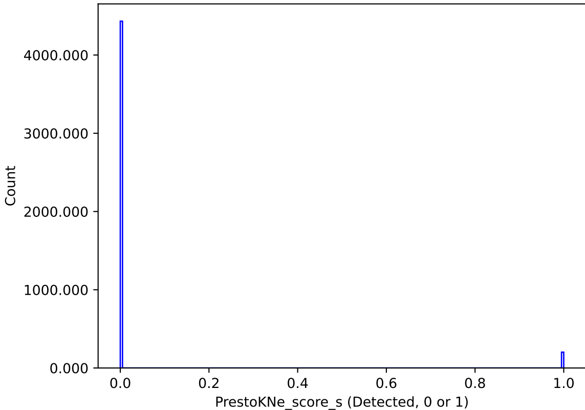
too_elab_r64_d2_gz_v3.4_10yrs : PrestoKNe_score_s
