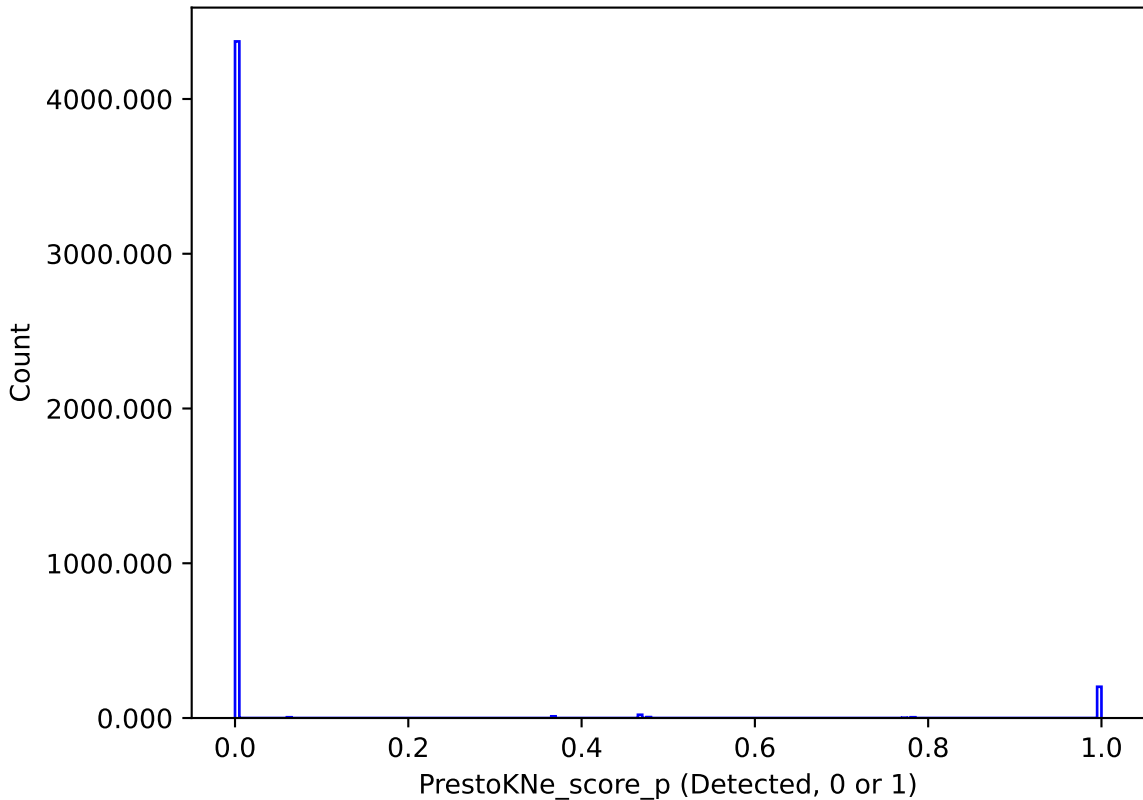
too_elab_r64_d2_gz_v3.4_10yrs : PrestoKNe_score_p
