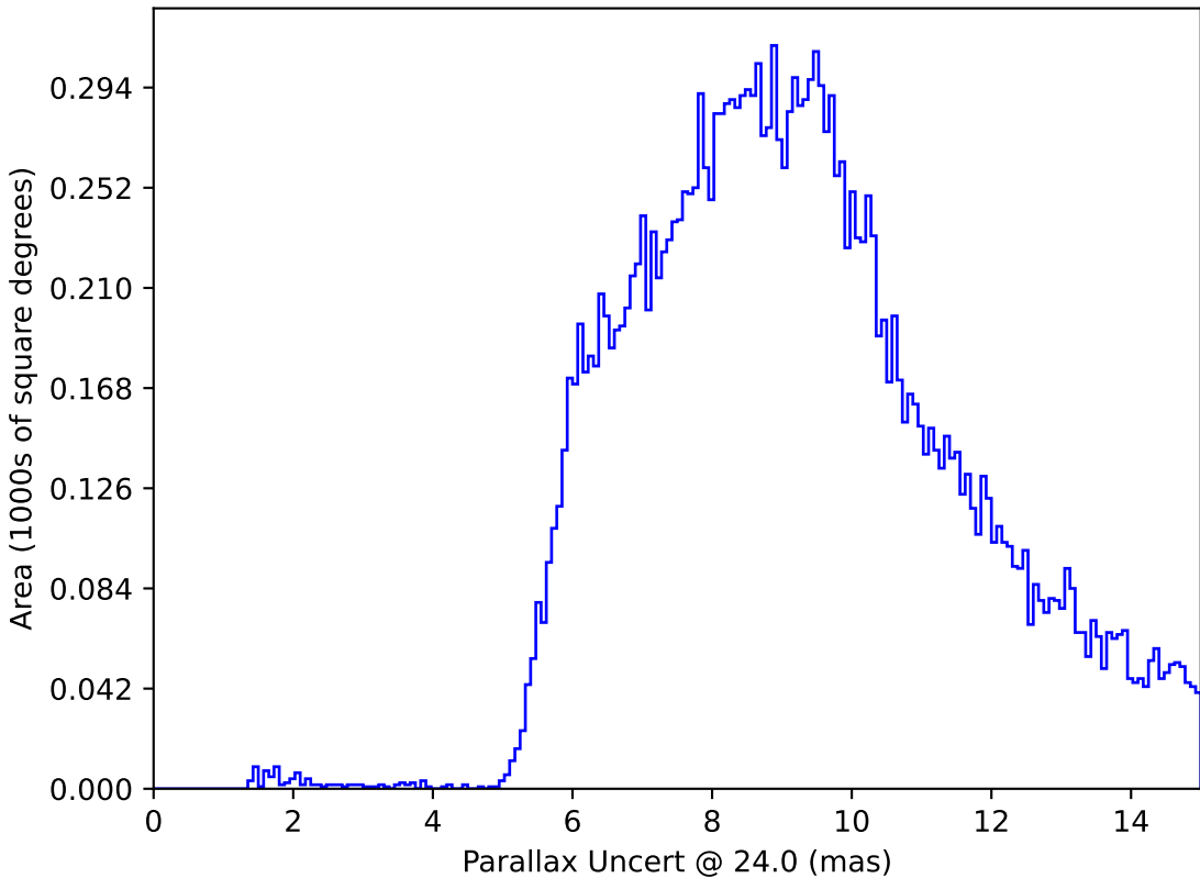
too_elab_r64_d2_gz_v3.4_10yrs : Parallax Uncert @ 24.0
