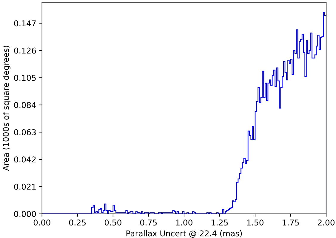
too_elab_r64_d2_gz_v3.4_10yrs : Parallax Uncert @ 22.4
