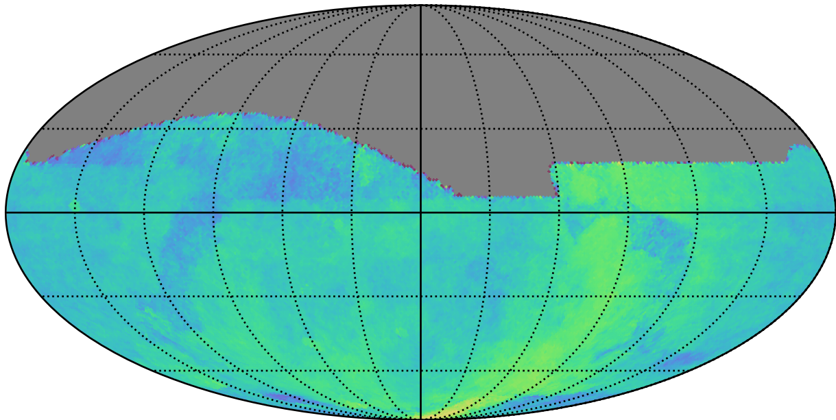
too_elab_r64_d2_gz_v3.4_10yrs : Parallax Coverage @ 24.0
