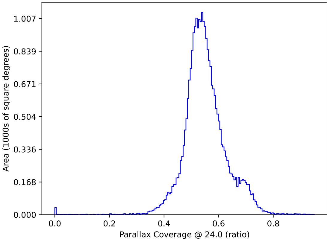
too_elab_r64_d2_gz_v3.4_10yrs : Parallax Coverage @ 24.0
