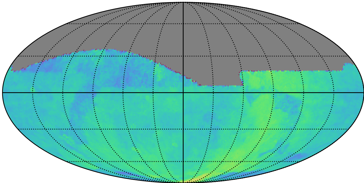
too_elab_r64_d2_gz_v3.4_10yrs : Parallax Coverage @ 22.4
