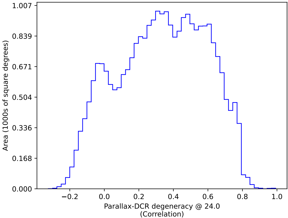
too_elab_r64_d2_gz_v3.4_10yrs : Parallax-DCR degeneracy @ 24.0
