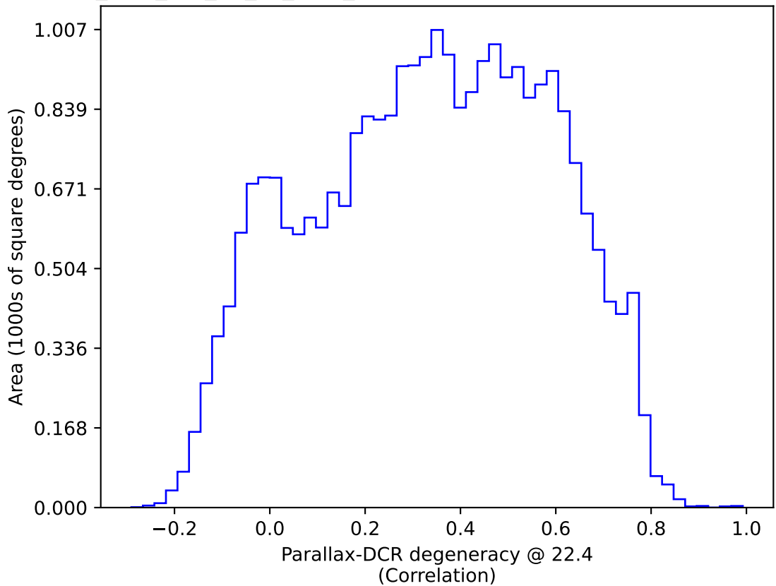
too_elab_r64_d2_gz_v3.4_10yrs : Parallax-DCR degeneracy @ 22.4
