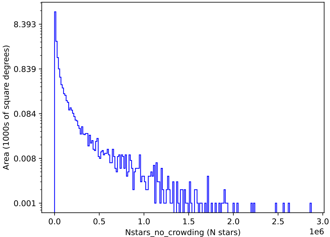
too_elab_r64_d2_gz_v3.4_10yrs u: Nstars_no_crowding
