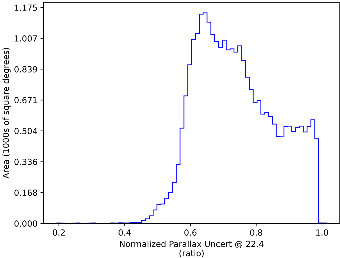
too_elab_r64_d2_gz_v3.4_10yrs : Normalized Parallax Uncert @ 22.4
