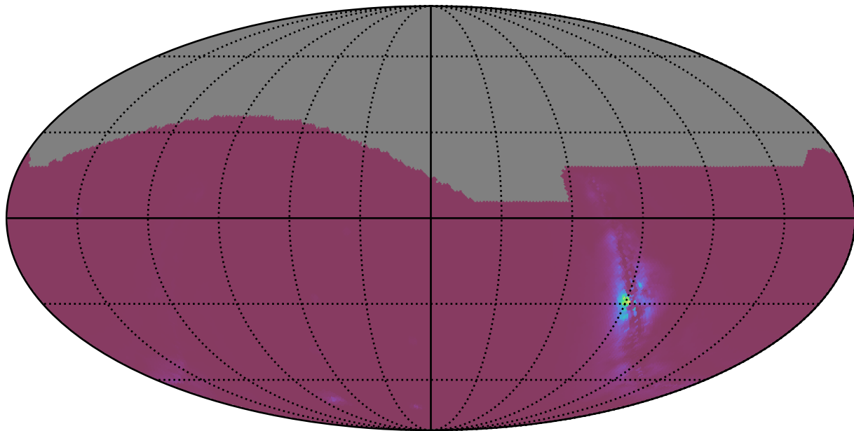
too_elab_r64_d2_gz_v3.4_10yrs : NlcPoints
