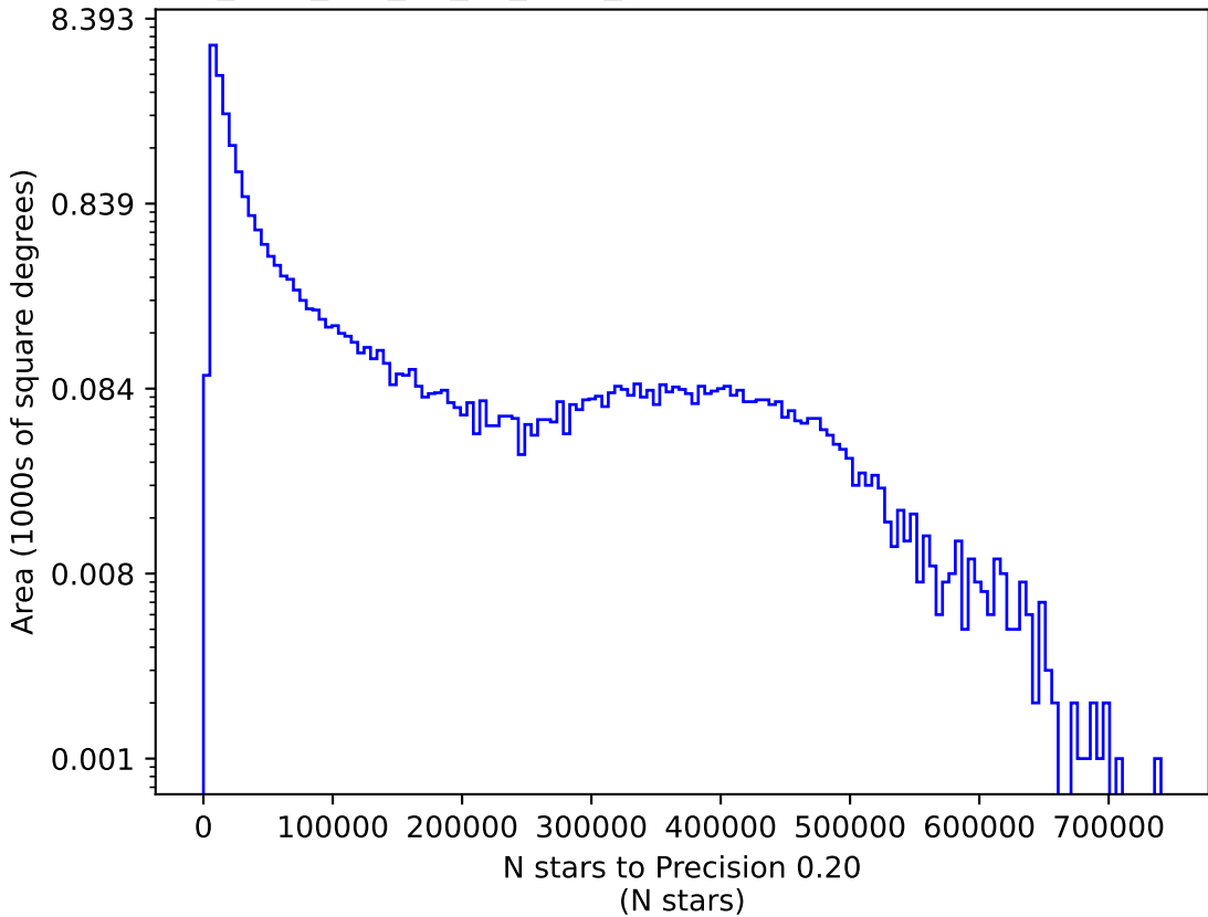
too_elab_r64_d2_gz_v3.4_10yrs z: N stars to Precision 0.20
